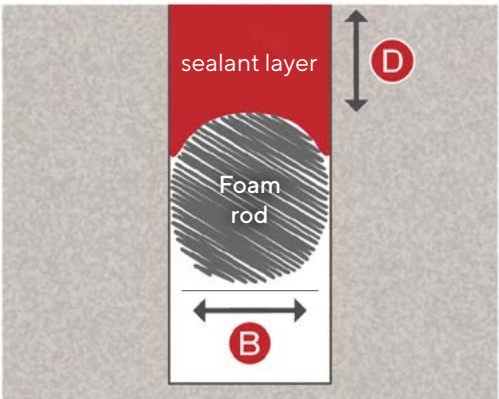
B= Joint width D= Joint depth
